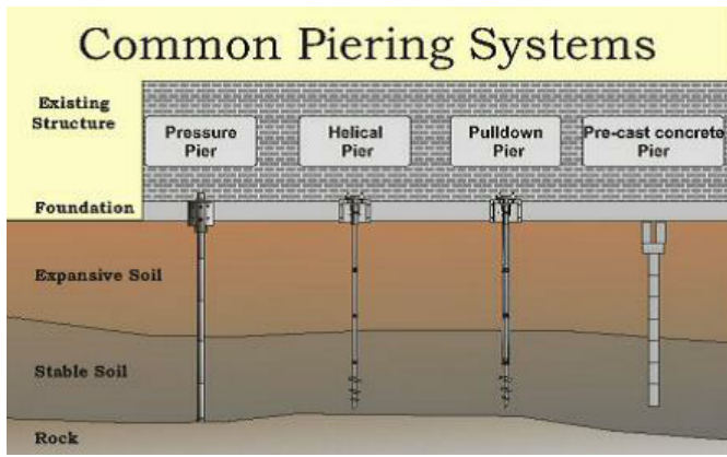
Piering System Diagram
